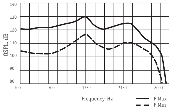
OSPL Response
