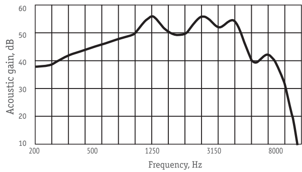
Full-on-gain Response
