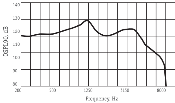
OSPL90 Response
