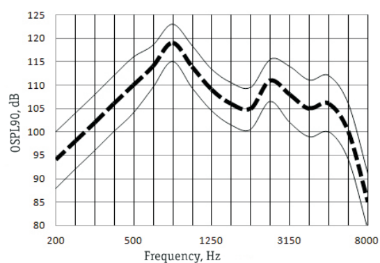
OSPL90 Response
