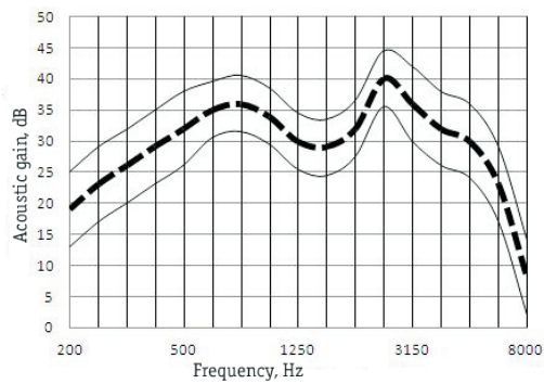
Full-On-Gain Response
