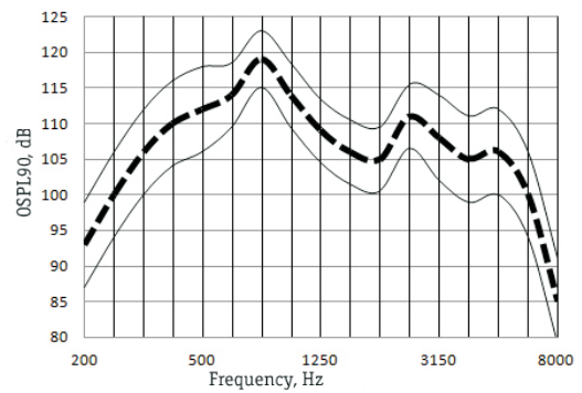
OSPL90 Response
