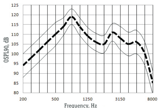
OSPL90 Response
