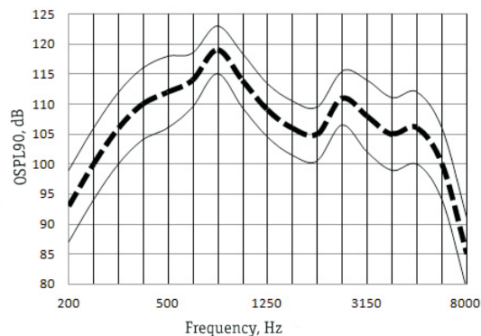
OSPL90 Response
