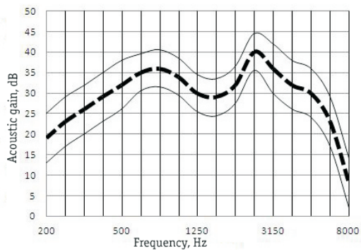
Full-On-Gain Response
