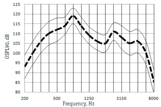
OSPL90 Response
