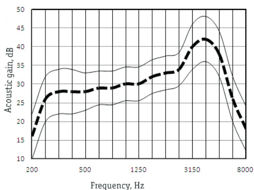
Full-On-Gain Response (wideband receiver)
