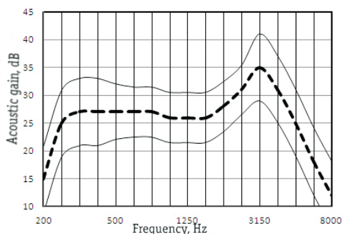
Full-On-Gain Response (standard receiver)
