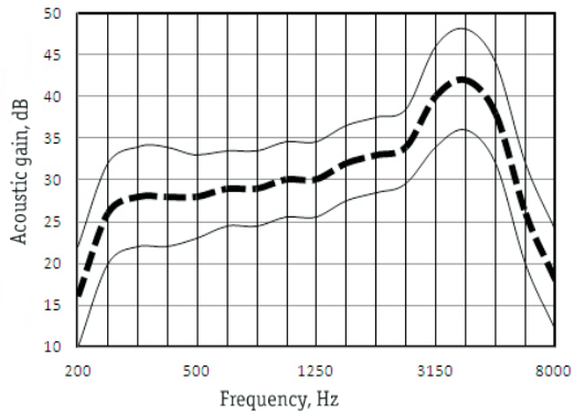
Full-On-Gain Response (wideband receiver)
