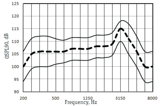
OSPL90 Response (wideband receiver)
