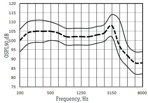
OSPL90 Response (standard receiver)
