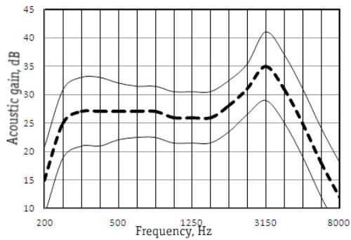
Full-On-Gain Response (wideband receiver)
