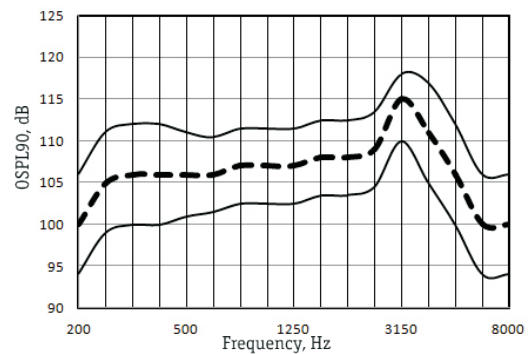
OSPL90 Response (wideband receiver)
