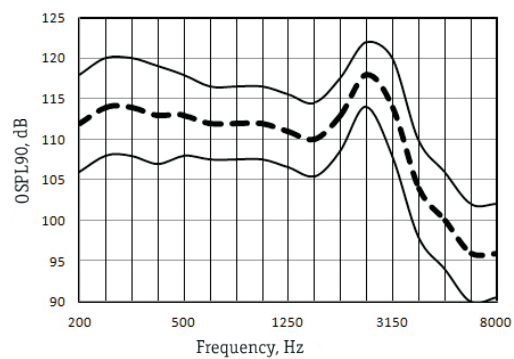
OSPL90 Response (wideband receiver)
