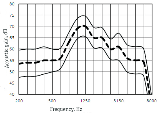
Full-On-Gain Response
