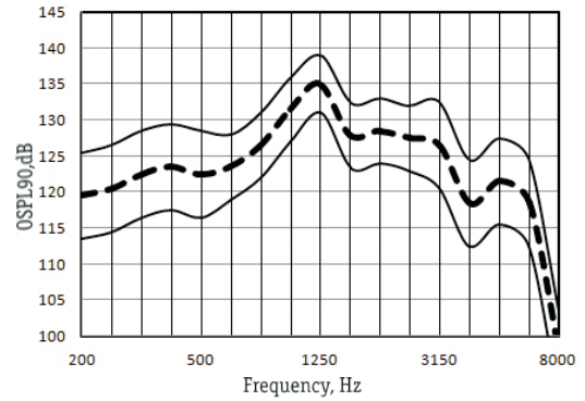
OSPL90 Response
