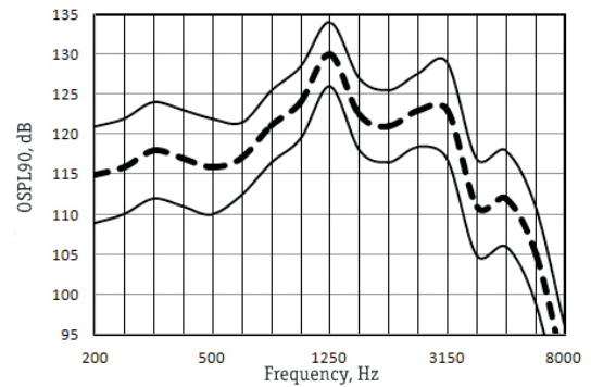
OSPL90 Response
