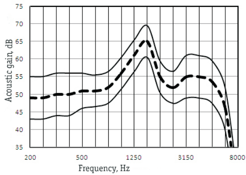
Full-On-Gain Response
