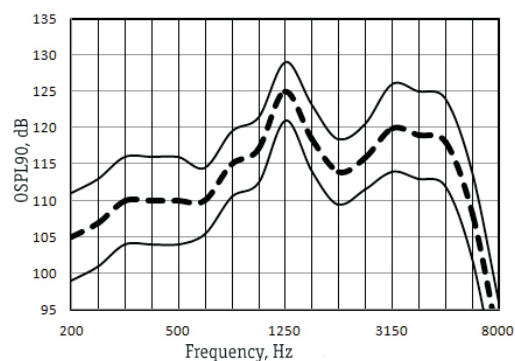
OSPL90 Response
