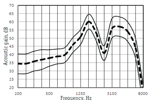
Full-On-Gain Response
