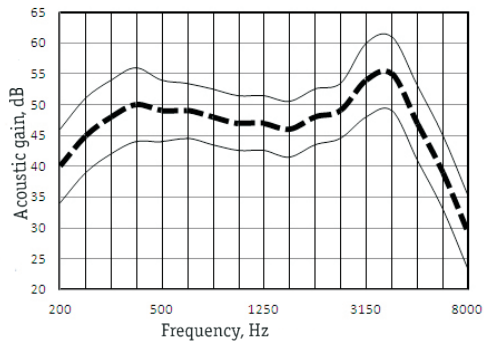
Full-On-Gain Response
