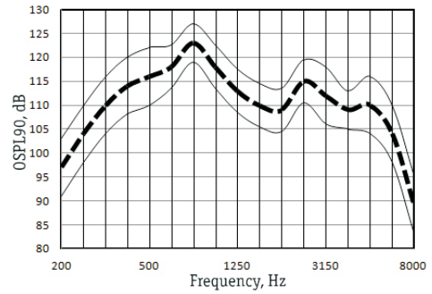
OSPL90 Response
