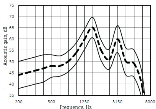
Full-On-Gain Response
