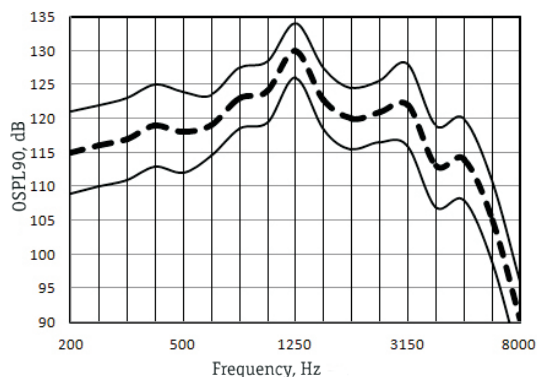
OSPL90 Response
