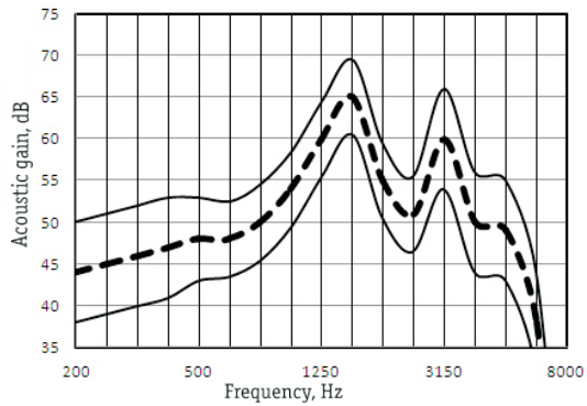
Full-On-Gain Response
