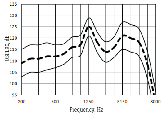
OSPL90 Response
