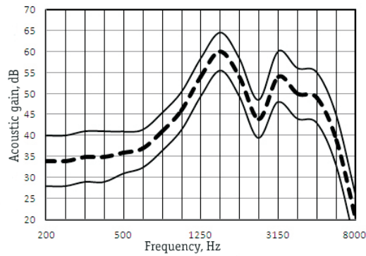
Full-On-Gain Response
